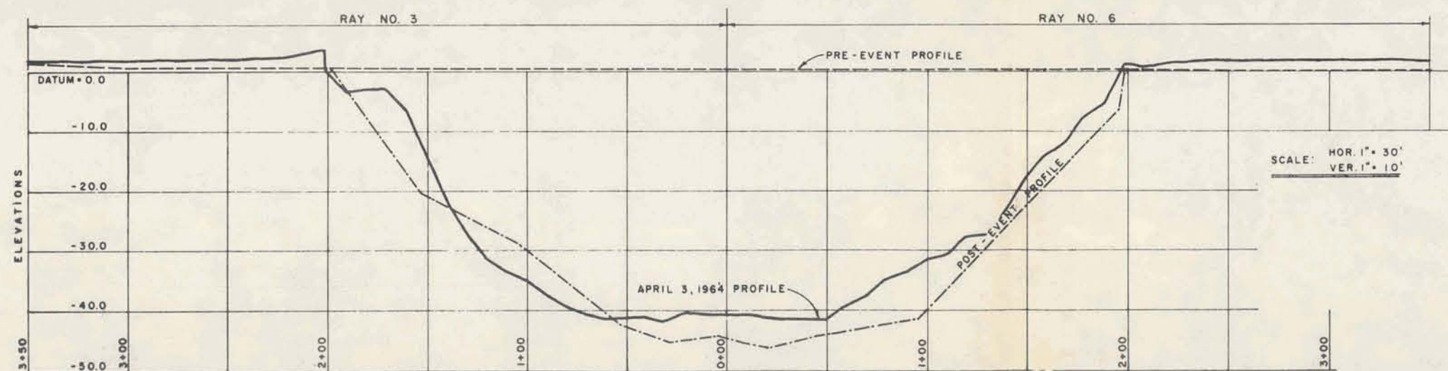
Fig. 19. Preshot, postshot, and 1964 survey profiles of Lacrosse crater.
